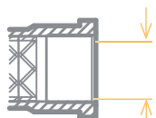
Inner diameter of the flange inlet housing: 24.3 mm / 0.958 inch
